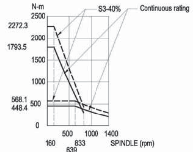
Torque Chart
