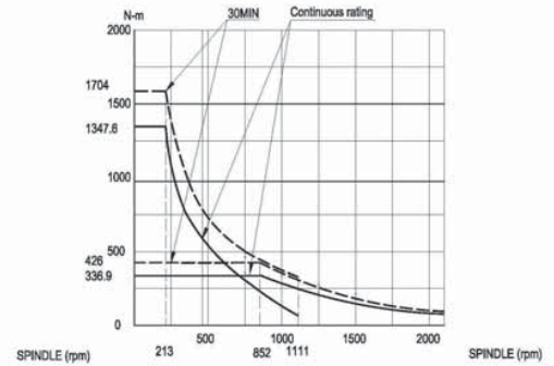
Torque Chart
