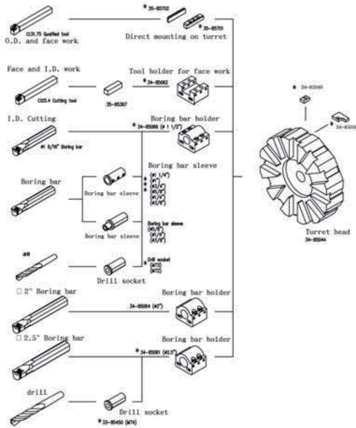
DUPLOMATIC VDI 50 COUPLING 1809 AXIAL TURRET
