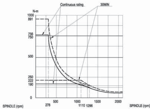
Torque Chart
