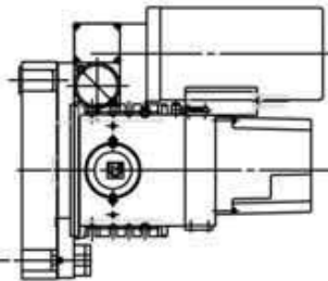
DUPLOMATIC VDI 50 COUPLING 1809 AXIAL TURRET
