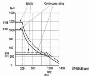
Torque Chart
